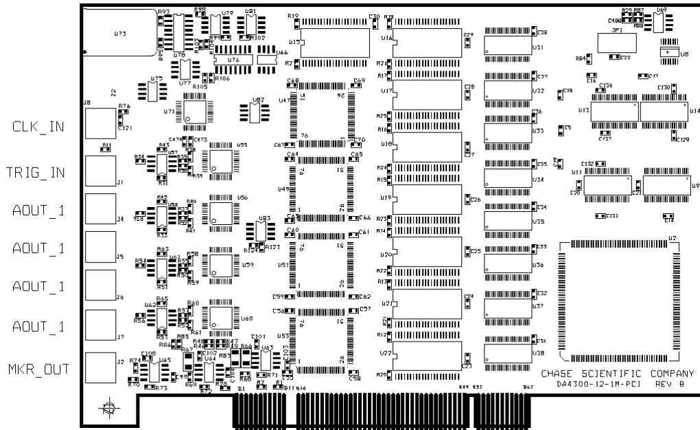
Figure 2 – Board Layout
